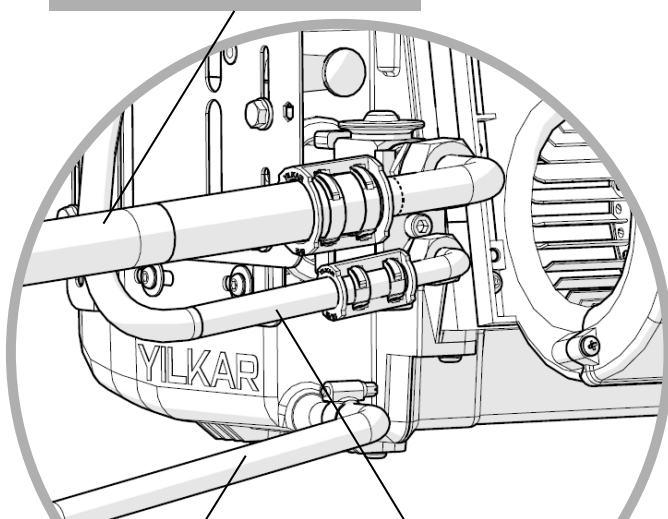
5/16 HOSE AND FITTING CONNECTION
